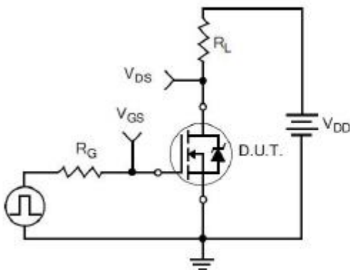
Figure 19. Resistive Switching Test Circuit
